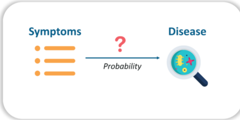
Bayesian Network
