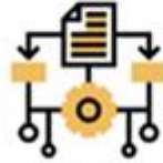
Fuzzy Logic
